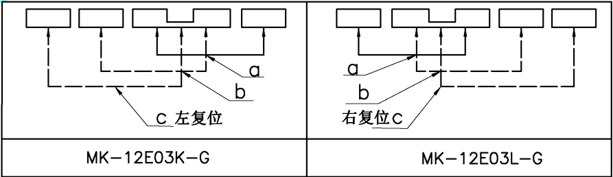
Schematic(Shorting)
