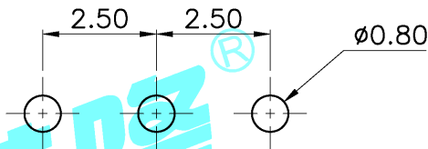
HOLE LAYOUT
